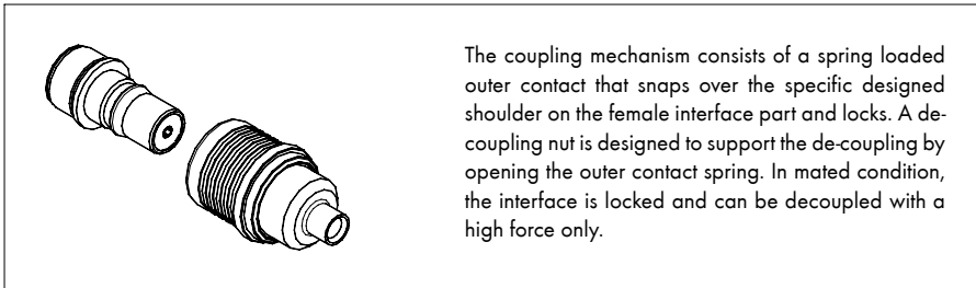
Figure 53 Quick-Lock coupling mechanism
