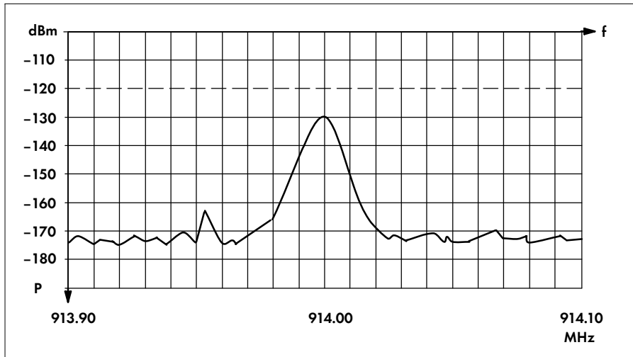
Figure 91 Result of the PIM measurement – related to frequency
