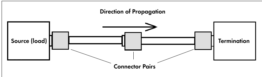
Figure 3 Direction of propagation along a RF line
