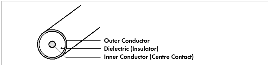
Figure 5 Construction of a RF line
